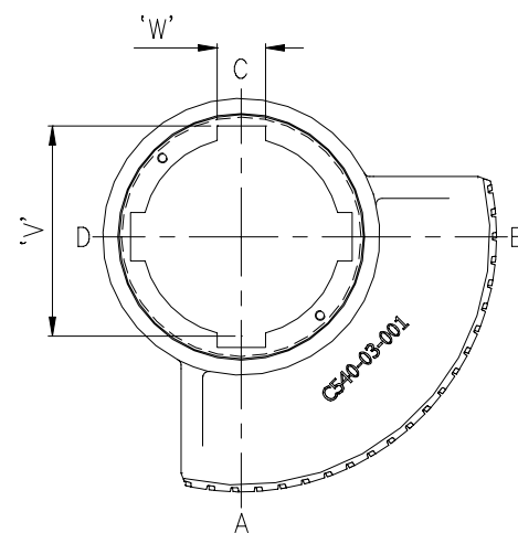
OUTPUT KEYWAY DETAILS SHOWN IN OPEN POSITION
