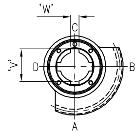
OUTPUT KEYWAY DETAILS SHOWN IN OPEN POSITION
