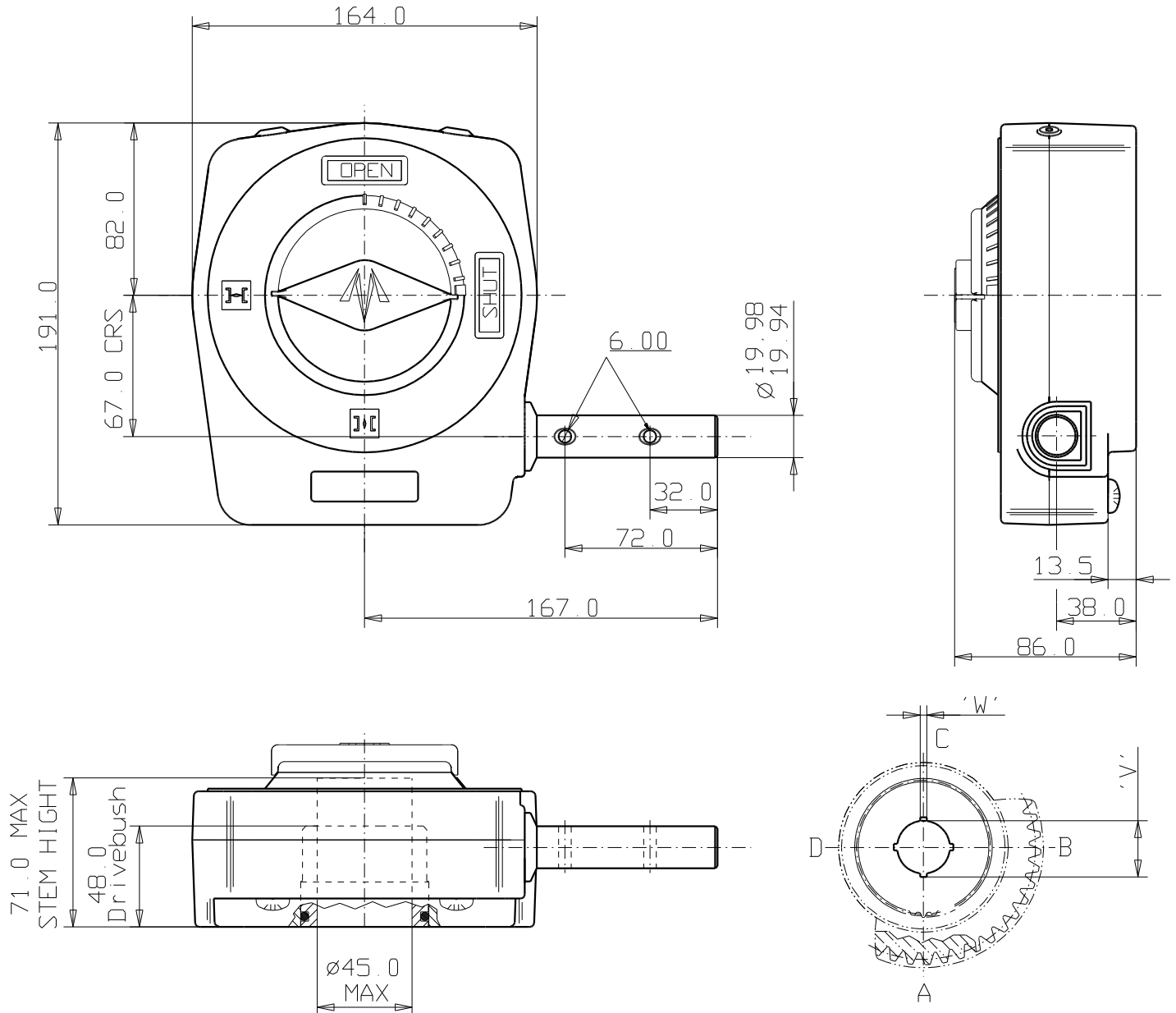
OUTPUT KEYWAY DETAILS (SHOWN IN OPEN POSITION)
